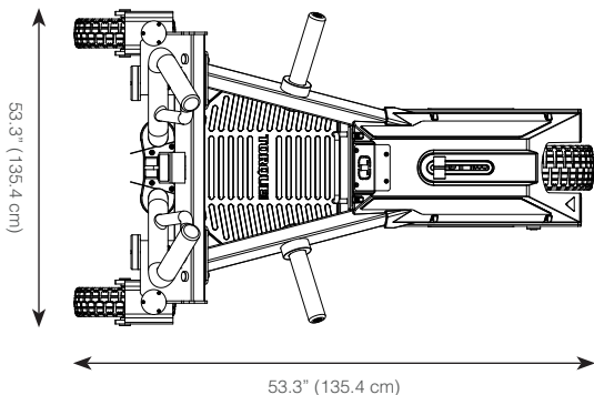
TOP VIEW - STANDARD
